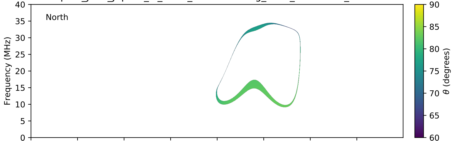
expres_juno_jupiter_io_isaac_lossc-wid1deg_3kev_20161019_v01.cdf
