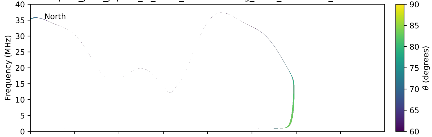
expres_juno_jupiter_io_isaac_lossc-wid1deg_3kev_20161018_v01.cdf
