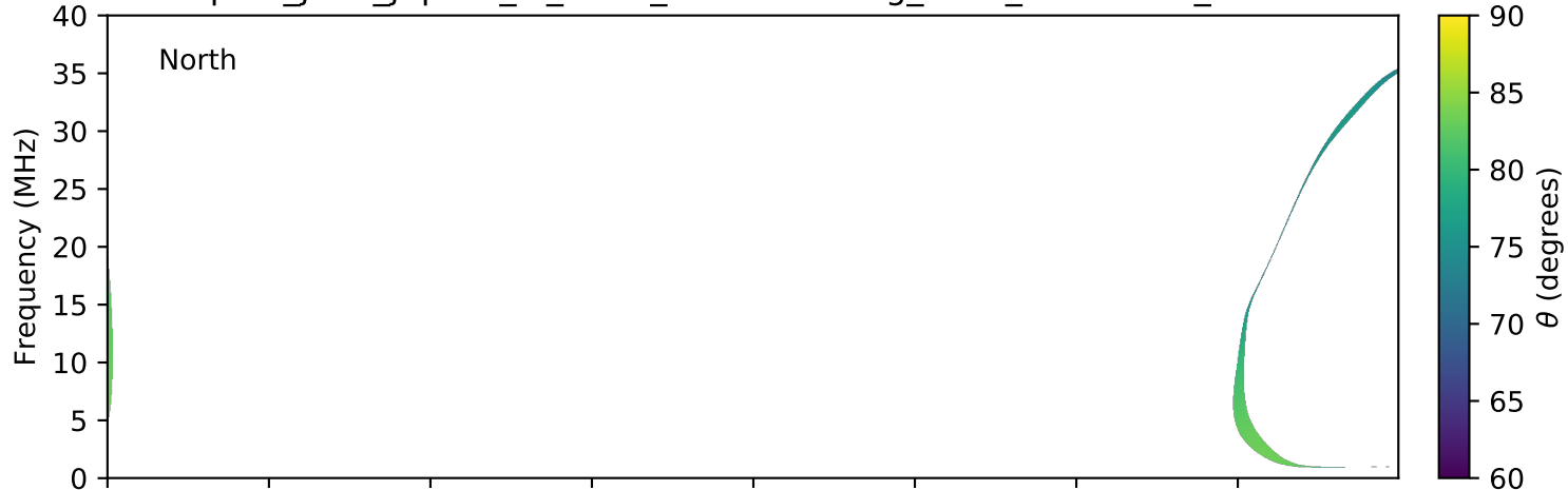
expres_juno_jupiter_io_isaac_lossc-wid1deg_3kev_20161017_v01.cdf
