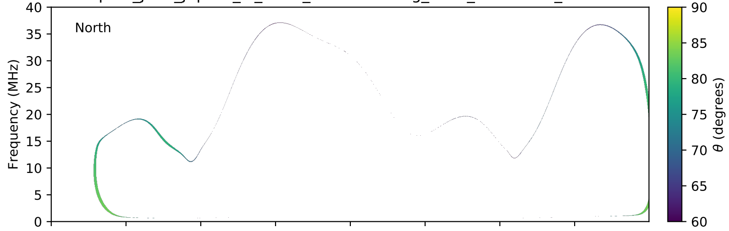
expres_juno_jupiter_io_isaac_lossc-wid1deg_3kev_20161016_v01.cdf
