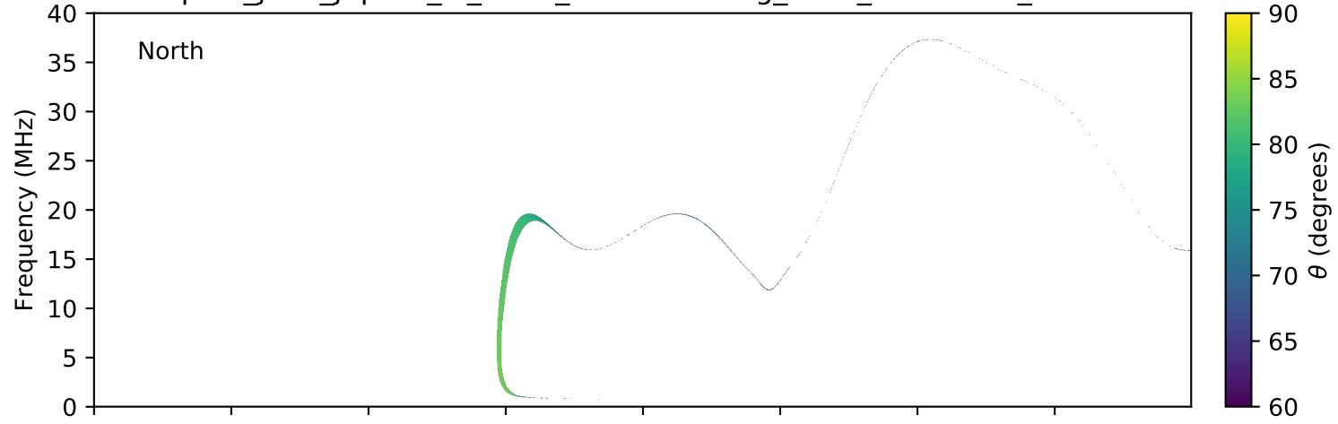
expres_juno_jupiter_io_isaac_lossc-wid1deg_3kev_20161014_v01.cdf
