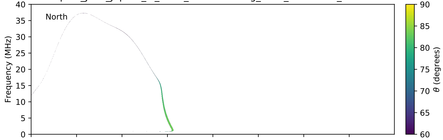
expres_juno_jupiter_io_isaac_lossc-wid1deg_3kev_20161013_v01.cdf
