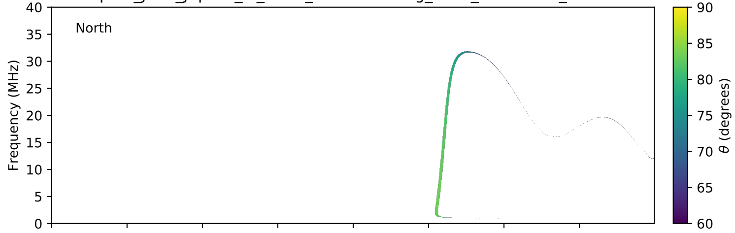
expres_juno_jupiter_io_isaac_lossc-wid1deg_3kev_20161012_v01.cdf
