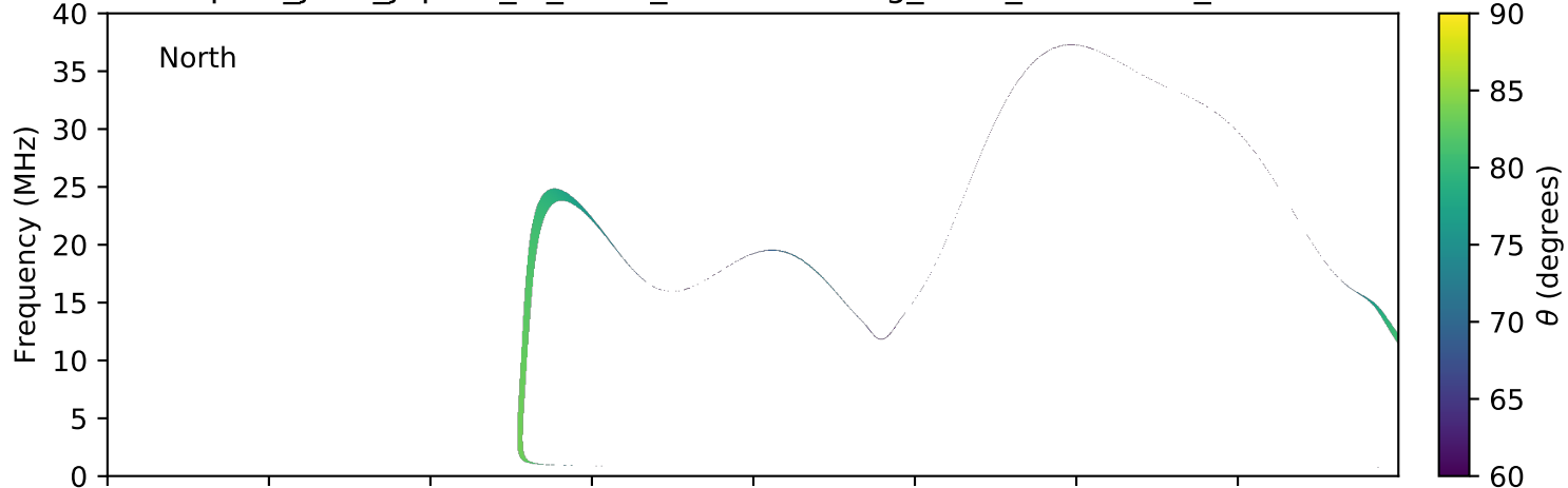
expres_juno_jupiter_io_isaac_lossc-wid1deg_3kev_20161007_v01.cdf
