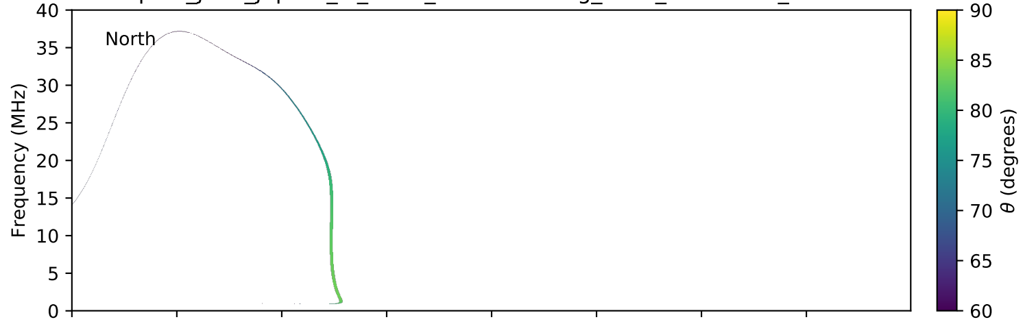
expres_juno_jupiter_io_isaac_lossc-wid1deg_3kev_20161006_v01.cdf
