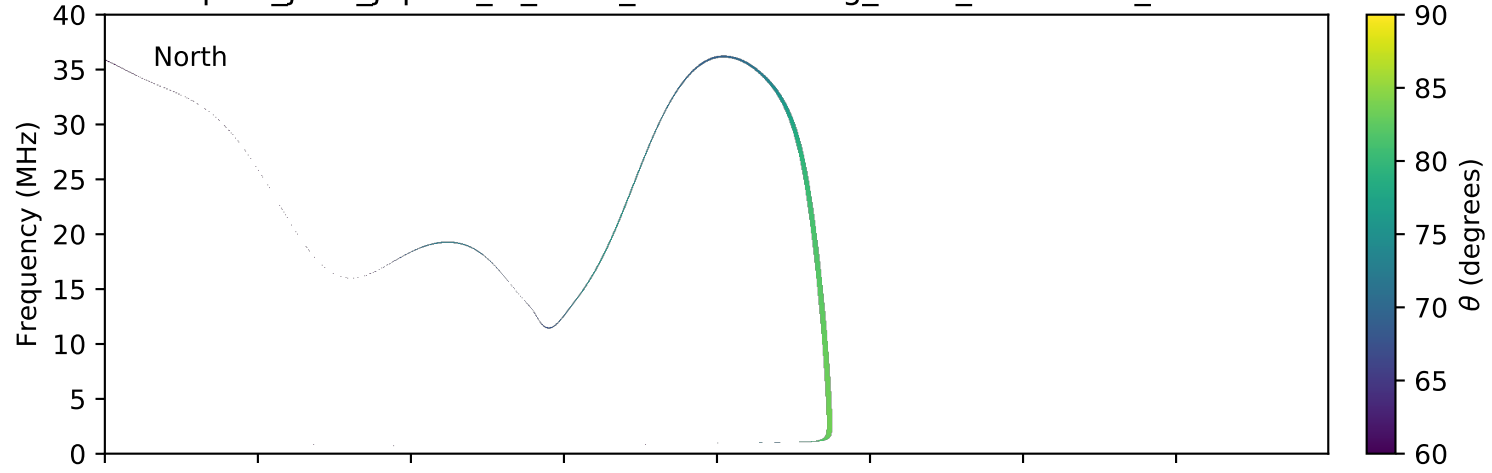
expres_juno_jupiter_io_isaac_lossc-wid1deg_3kev_20161004_v01.cdf
