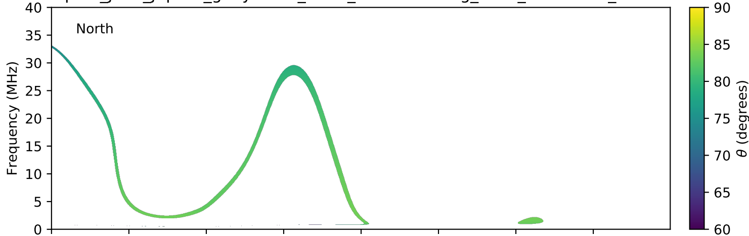
expres_juno_jupiter_ganymede_isaac_lossc-wid1deg_3kev_20161031_v01.cdf
