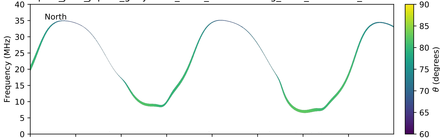
expres_juno_jupiter_ganymede_isaac_lossc-wid1deg_3kev_20161030_v01.cdf
