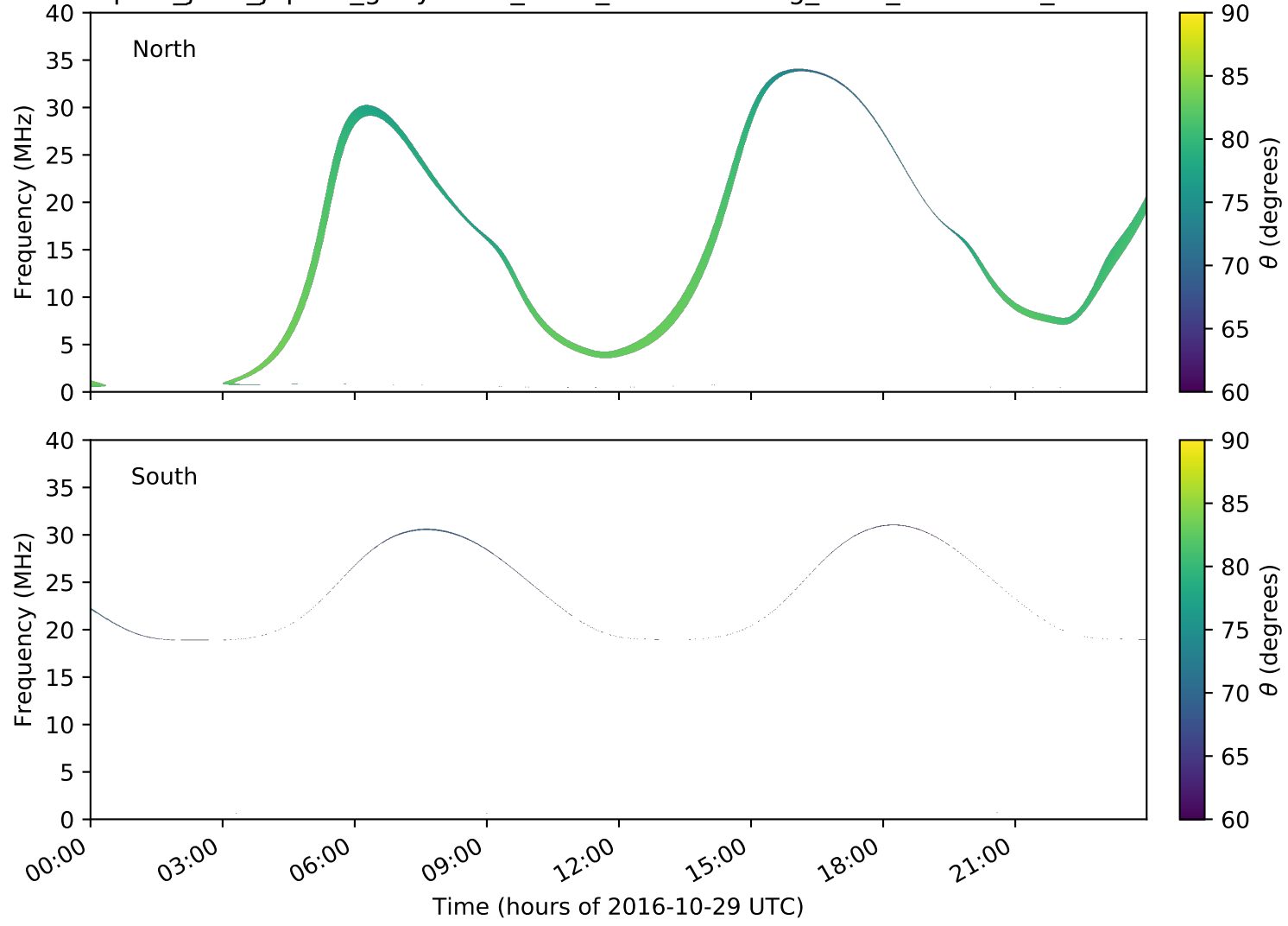
expres_juno_jupiter_ganymede_isaac_lossc-wid1deg_3kev_20161029_v01.cdf
