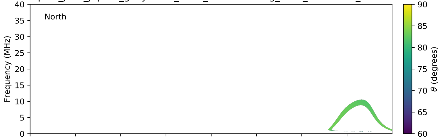
expres_juno_jupiter_ganymede_isaac_lossc-wid1deg_3kev_20161028_v01.cdf
