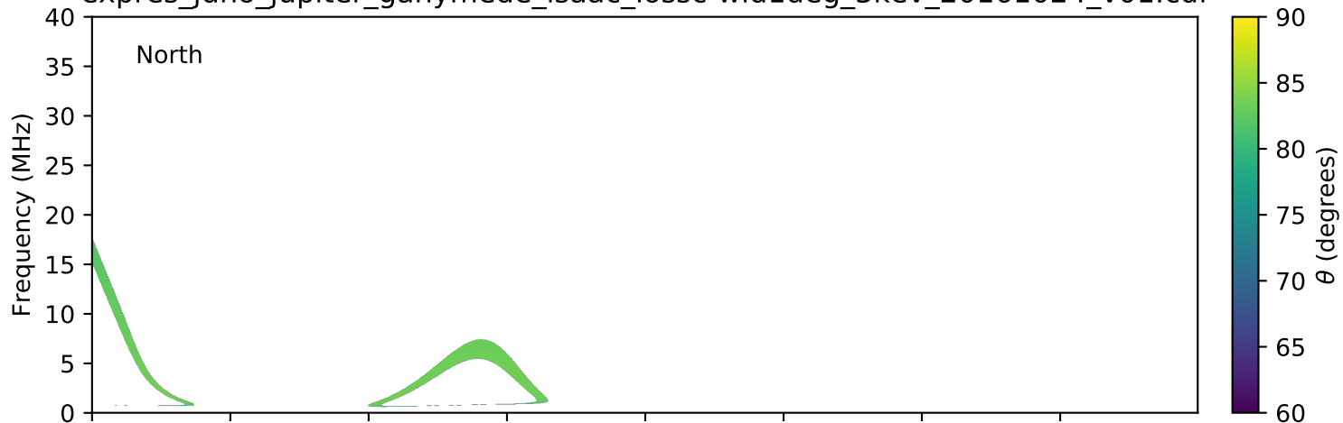
expres_juno_jupiter_ganymede_isaac_lossc-wid1deg_3kev_20161024_v01.cdf
