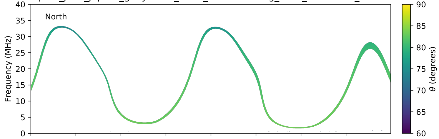
expres_juno_jupiter_ganymede_isaac_lossc-wid1deg_3kev_20161023_v01.cdf
