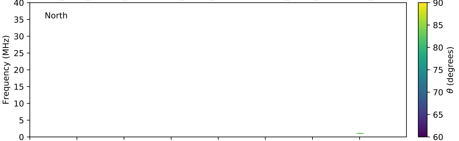
expres_juno_jupiter_ganymede_isaac_lossc-wid1deg_3kev_20161021_v01.cdf
