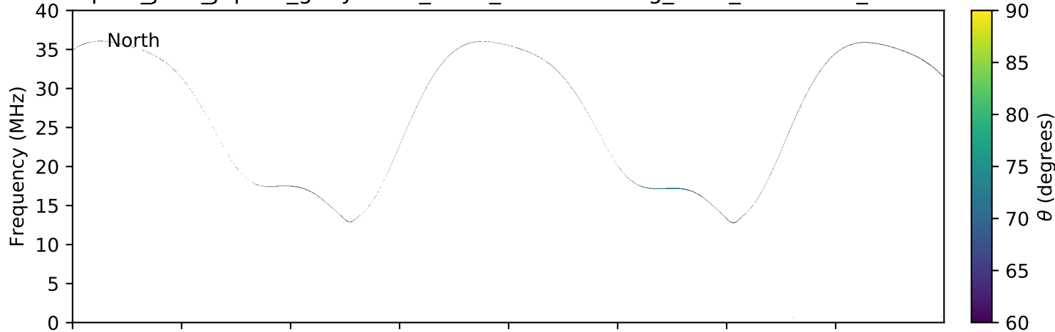
expres_juno_jupiter_ganymede_isaac_lossc-wid1deg_3kev_20161016_v01.cdf
