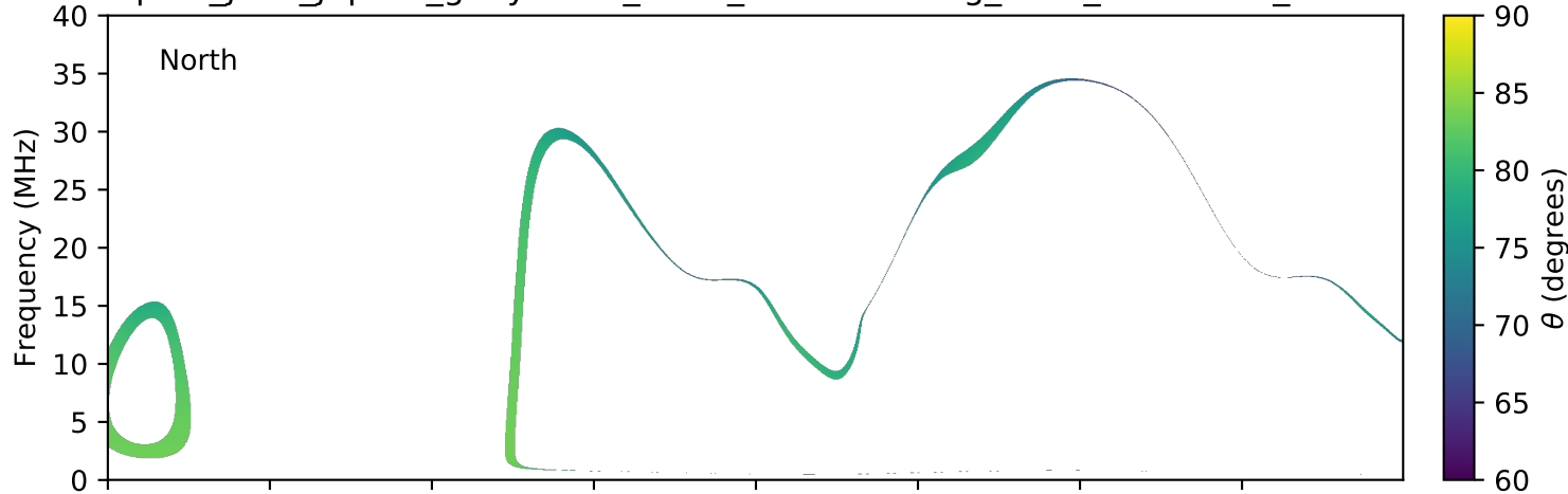
expres_juno_jupiter_ganymede_isaac_lossc-wid1deg_3kev_20161014_v01.cdf
