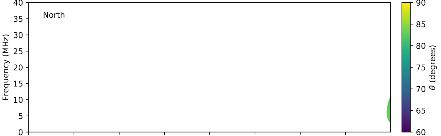
expres_juno_jupiter_ganymede_isaac_lossc-wid1deg_3kev_20161013_v01.cdf
