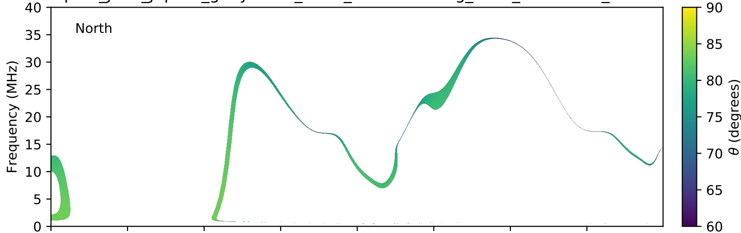
expres_juno_jupiter_ganymede_isaac_lossc-wid1deg_3kev_20161007_v01.cdf
