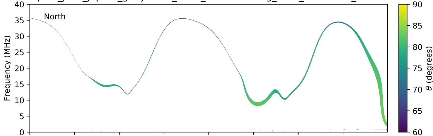
expres_juno_jupiter_ganymede_isaac_lossc-wid1deg_3kev_20161002_v01.cdf
