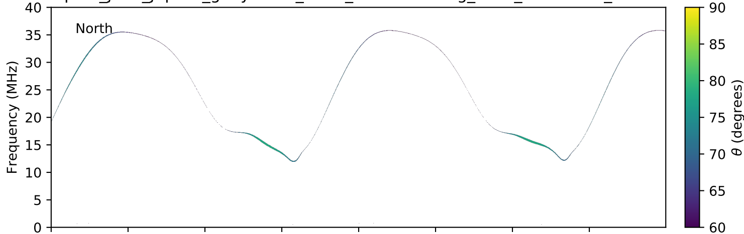
expres_juno_jupiter_ganymede_isaac_lossc-wid1deg_3kev_20161001_v01.cdf
