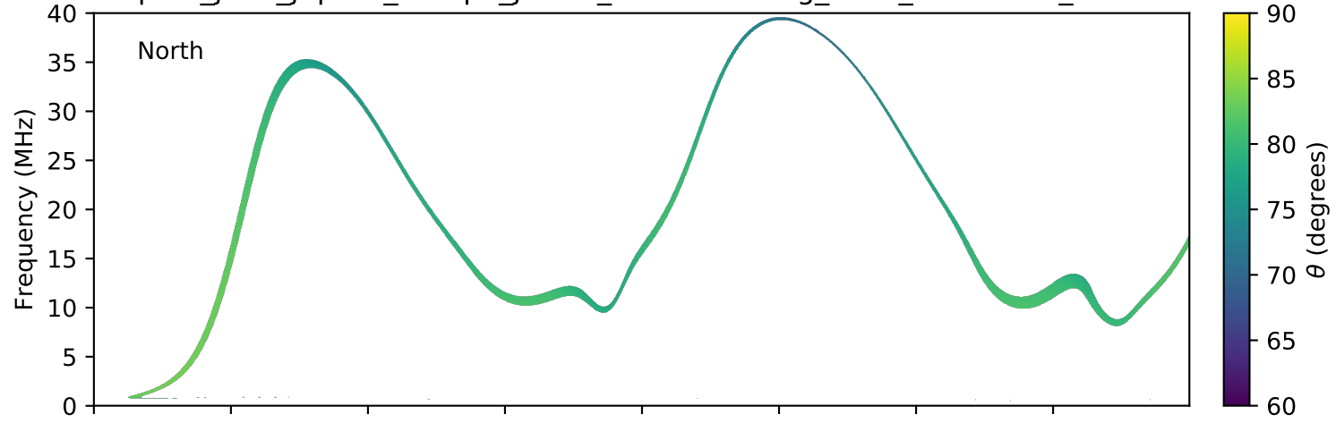
expres_juno_jupiter_europa_jrm09_lossc-wid1deg_3kev_20161027_v01.cdf
