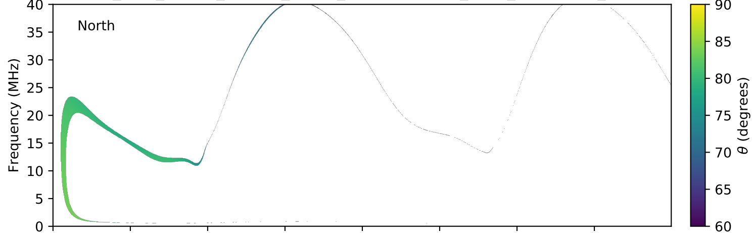
expres_juno_jupiter_europa_jrm09_lossc-wid1deg_3kev_20161016_v01.cdf
