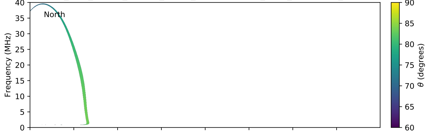
expres_juno_jupiter_europa_jrm09_lossc-wid1deg_3kev_20161014_v01.cdf
