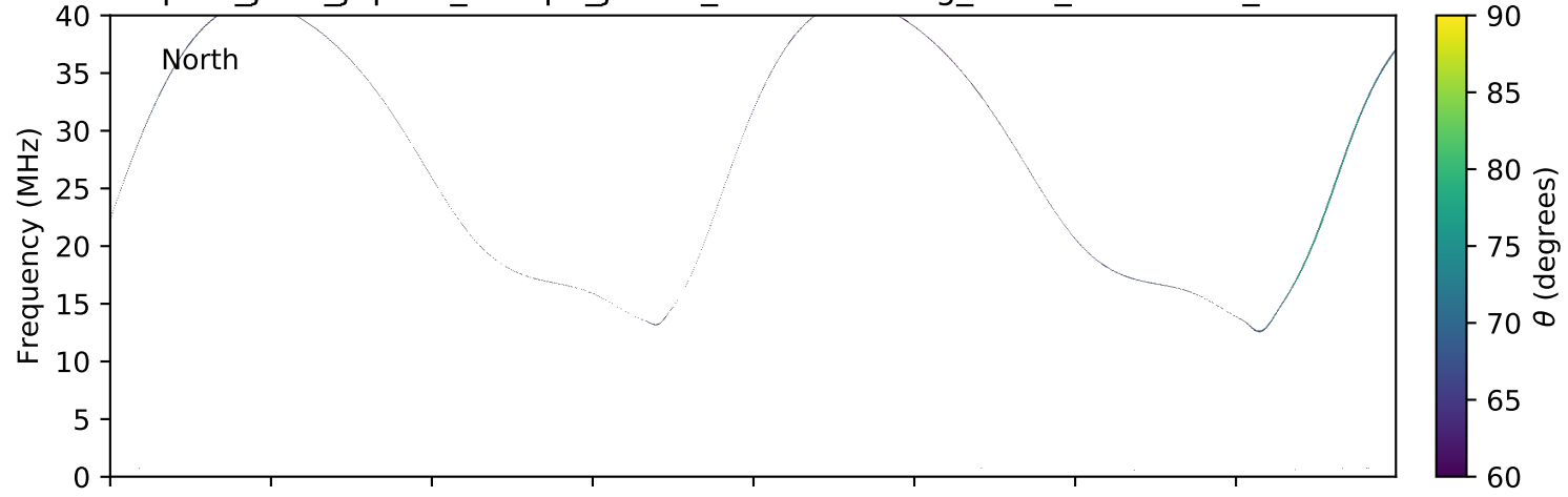
expres_juno_jupiter_europa_jrm09_lossc-wid1deg_3kev_20161013_v01.cdf
