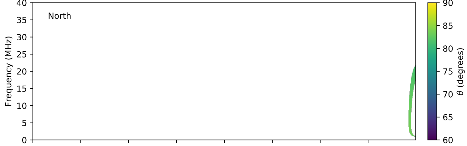
expres_juno_jupiter_europa_jrm09_lossc-wid1deg_3kev_20161008_v01.cdf
