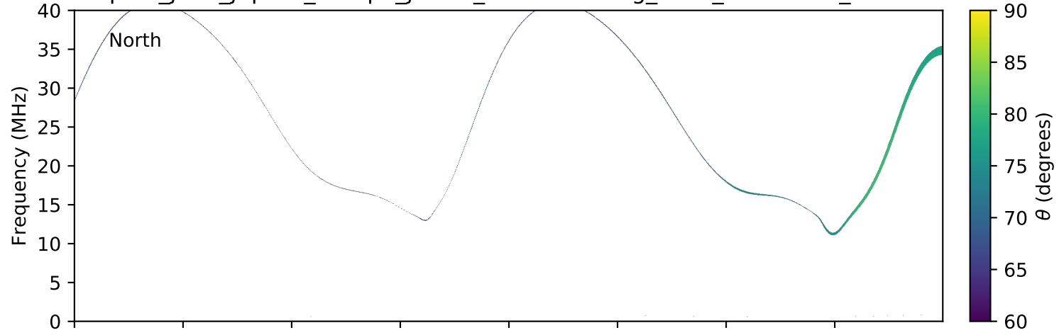
expres_juno_jupiter_europa_jrm09_lossc-wid1deg_3kev_20161006_v01.cdf
