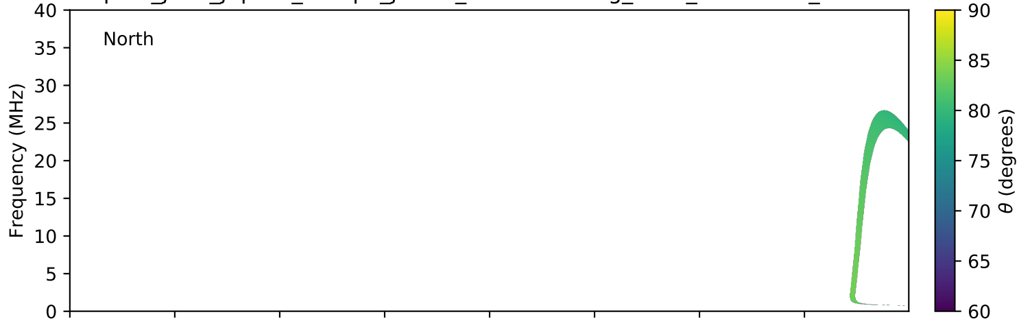
expres_juno_jupiter_europa_jrm09_lossc-wid1deg_3kev_20161001_v01.cdf
