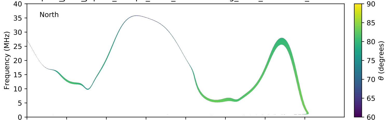
expres_juno_jupiter_europa_isaac_lossc-wid1deg_3kev_20161031_v01.cdf
