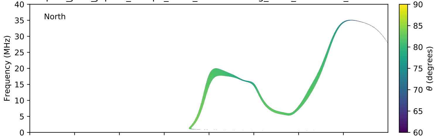
expres_juno_jupiter_europa_isaac_lossc-wid1deg_3kev_20161030_v01.cdf
