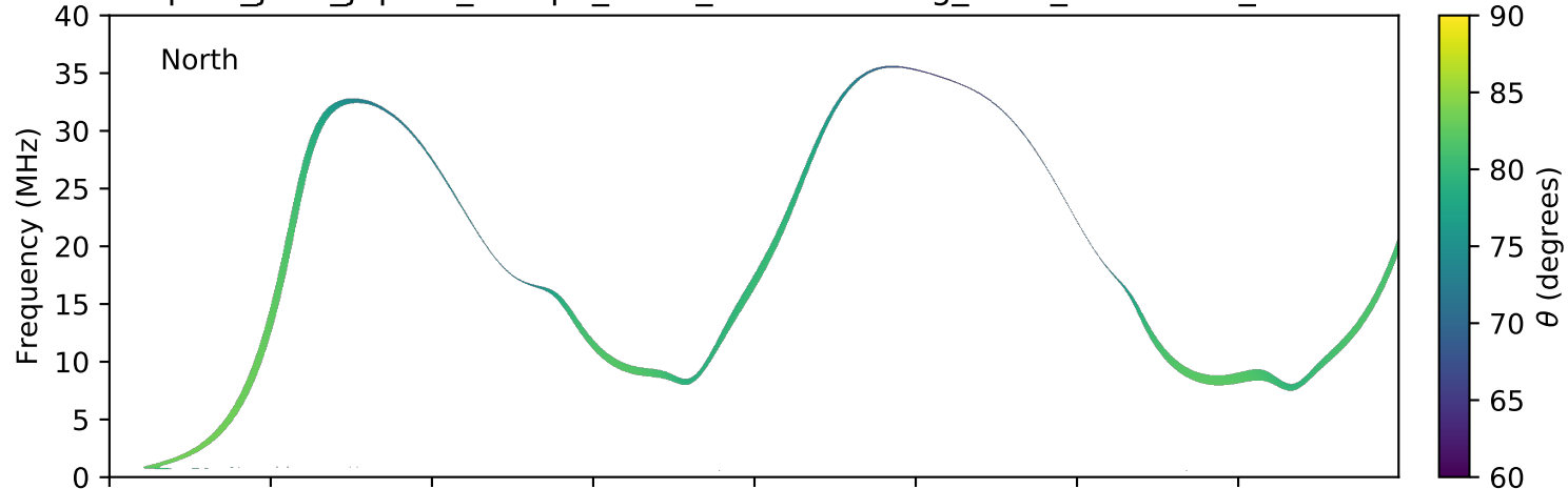
expres_juno_jupiter_europa_isaac_lossc-wid1deg_3kev_20161027_v01.cdf
