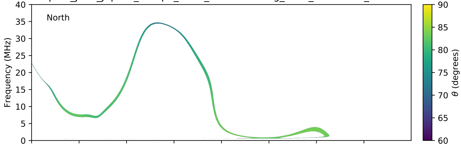
expres_juno_jupiter_europa_isaac_lossc-wid1deg_3kev_20161024_v01.cdf
