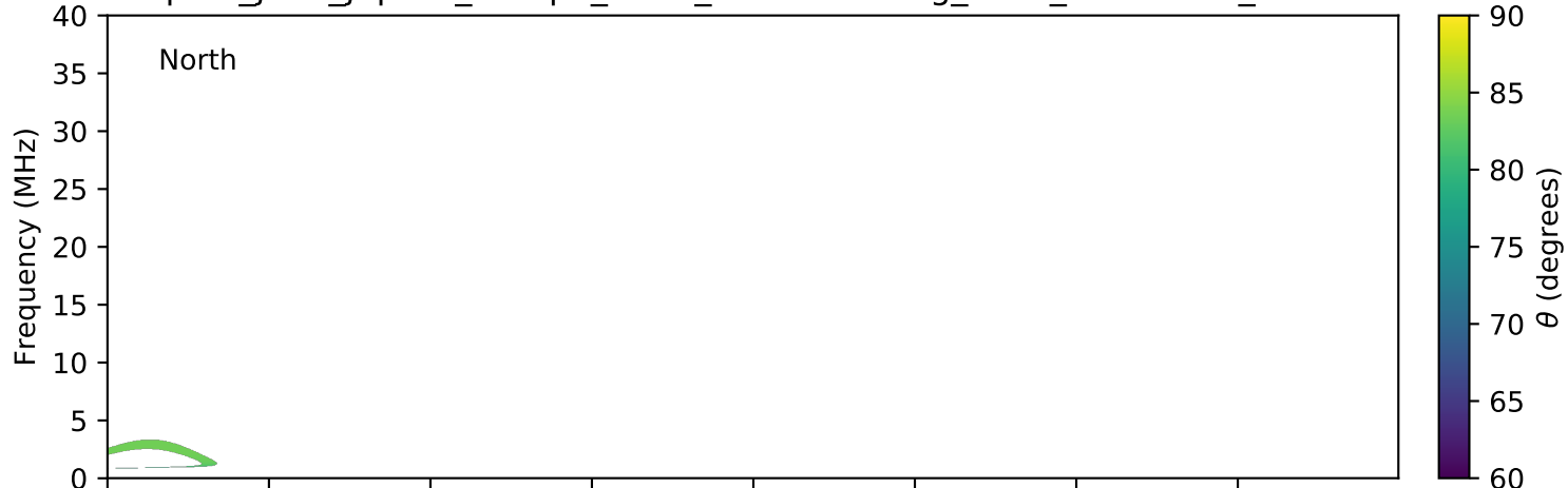
expres_juno_jupiter_europa_isaac_lossc-wid1deg_3kev_20161021_v01.cdf
