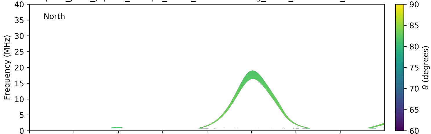
expres_juno_jupiter_europa_isaac_lossc-wid1deg_3kev_20161020_v01.cdf
