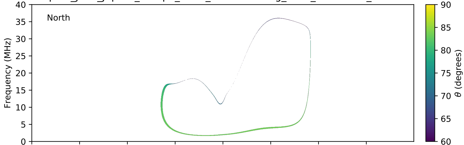
expres_juno_jupiter_europa_isaac_lossc-wid1deg_3kev_20161019_v01.cdf
