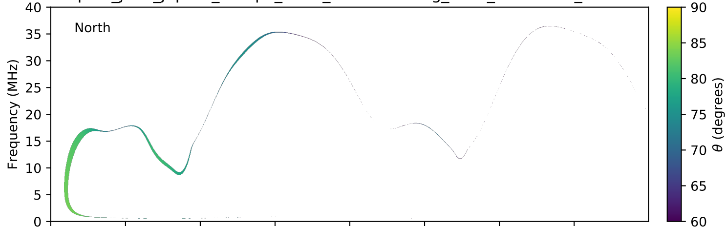
expres_juno_jupiter_europa_isaac_lossc-wid1deg_3kev_20161016_v01.cdf
