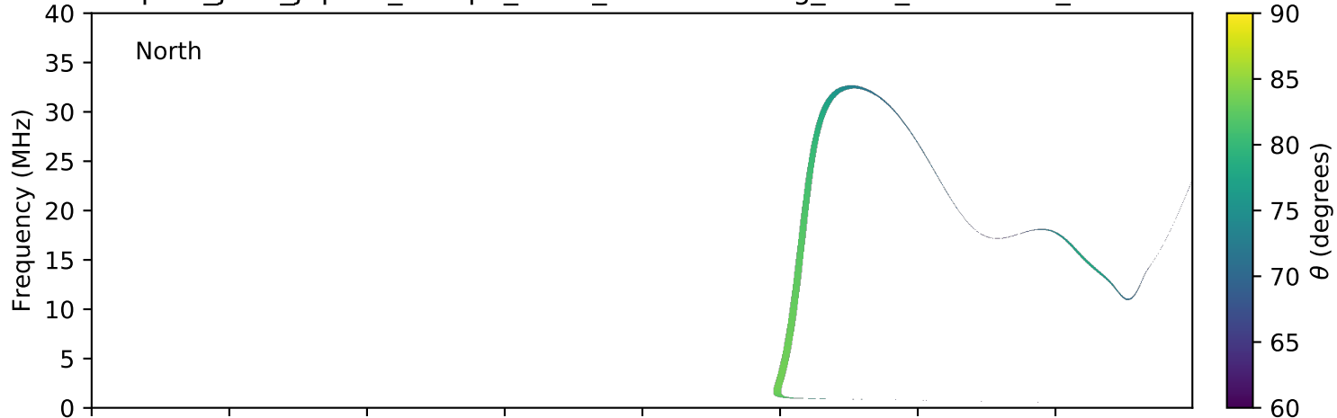
expres_juno_jupiter_europa_isaac_lossc-wid1deg_3kev_20161012_v01.cdf
