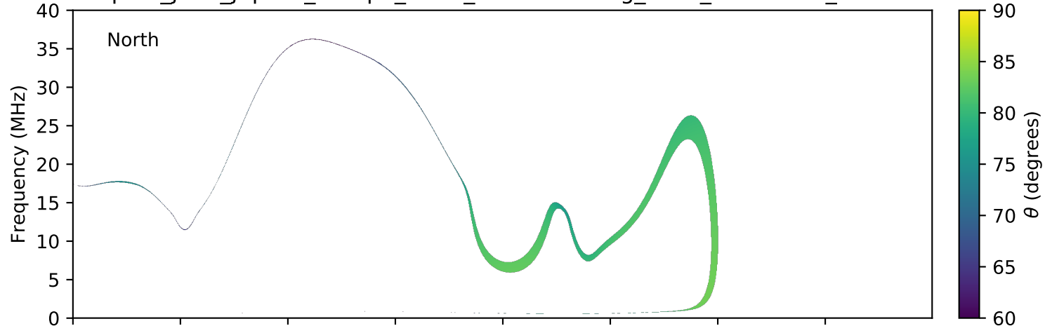
expres_juno_jupiter_europa_isaac_lossc-wid1deg_3kev_20161010_v01.cdf
