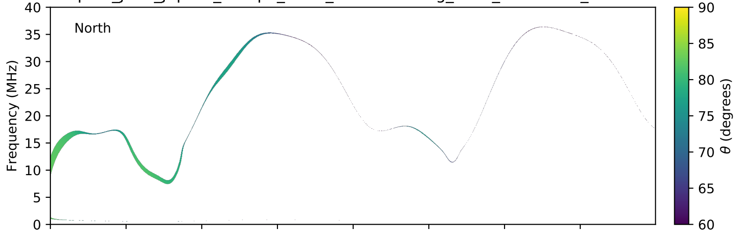
expres_juno_jupiter_europa_isaac_lossc-wid1deg_3kev_20161009_v01.cdf
