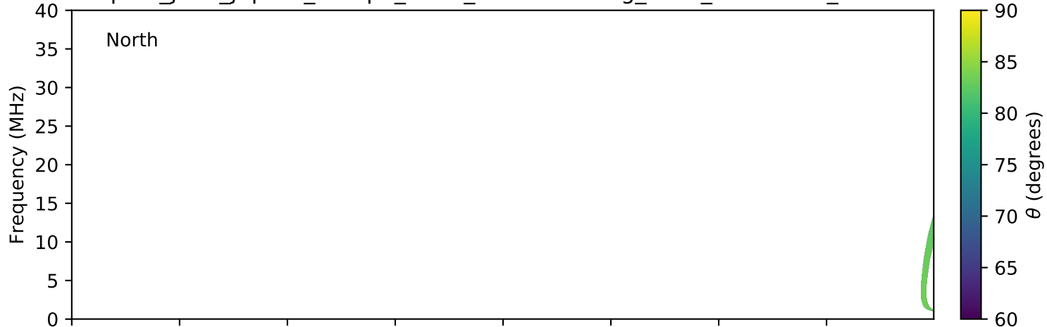
expres_juno_jupiter_europa_isaac_lossc-wid1deg_3kev_20161008_v01.cdf
