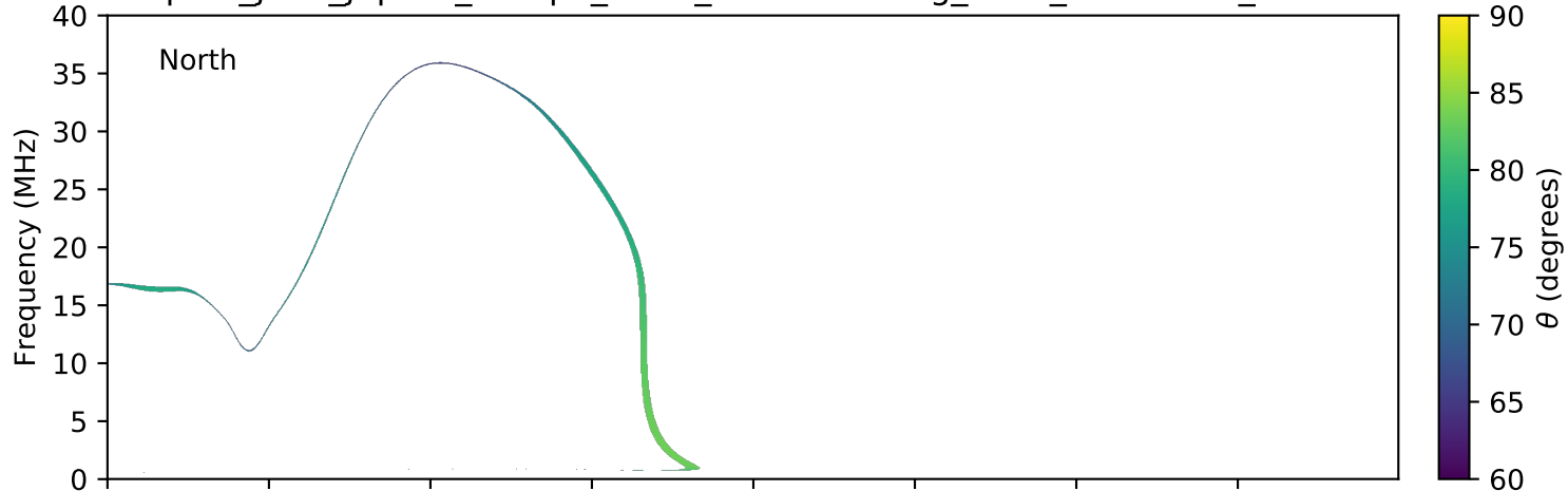
expres_juno_jupiter_europa_isaac_lossc-wid1deg_3kev_20161003_v01.cdf
