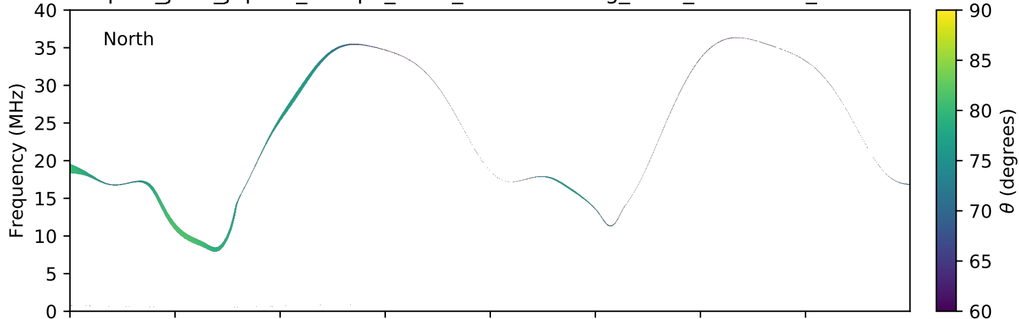
expres_juno_jupiter_europa_isaac_lossc-wid1deg_3kev_20161002_v01.cdf
