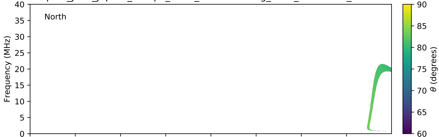
expres_juno_jupiter_europa_isaac_lossc-wid1deg_3kev_20161001_v01.cdf
