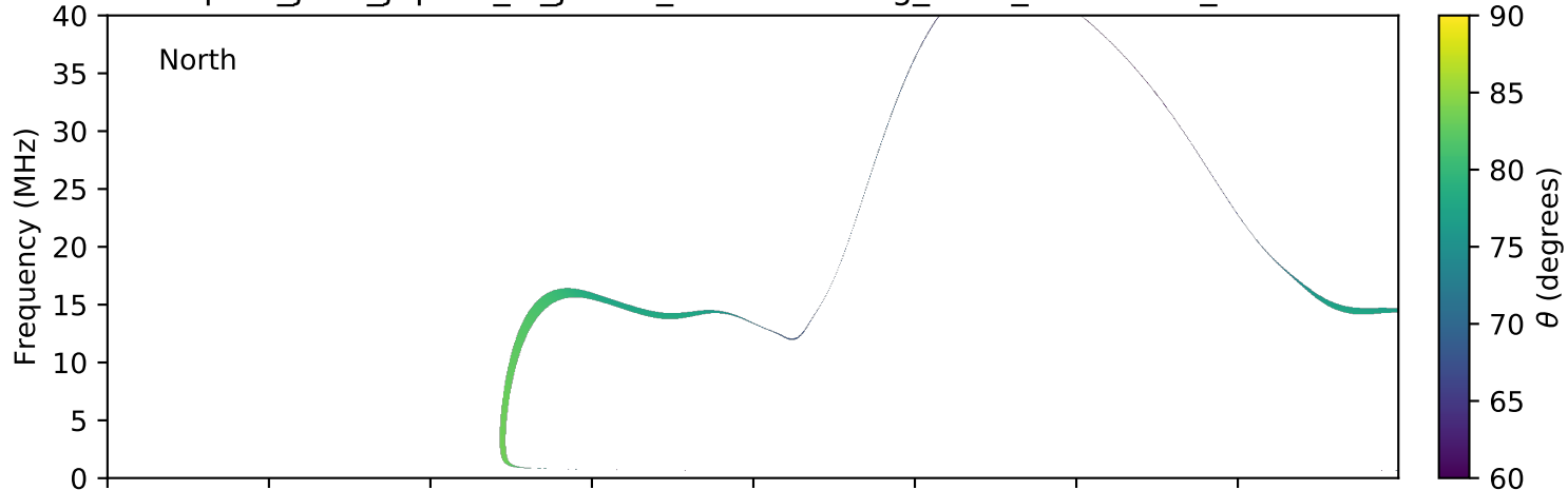
expres_juno_jupiter_io_jrm09_lossc-wid1deg_3kev_20160730_v01.cdf
