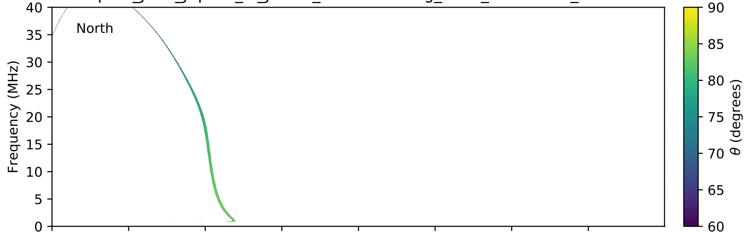
expres_juno_jupiter_io_jrm09_lossc-wid1deg_3kev_20160729_v01.cdf
