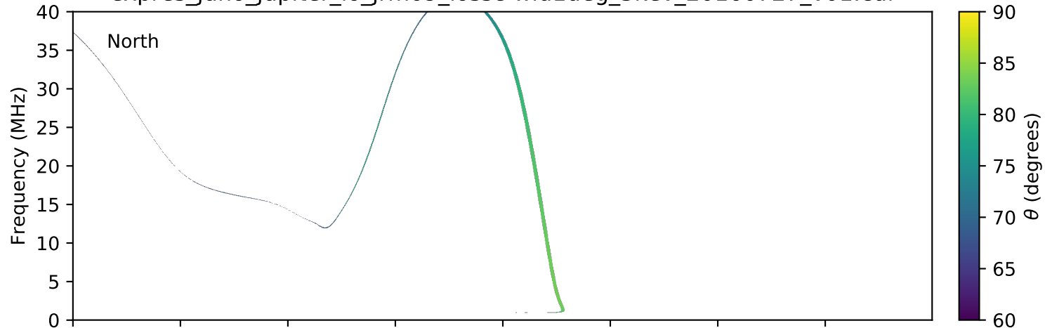
expres_juno_jupiter_io_jrm09_lossc-wid1deg_3kev_20160727_v01.cdf
