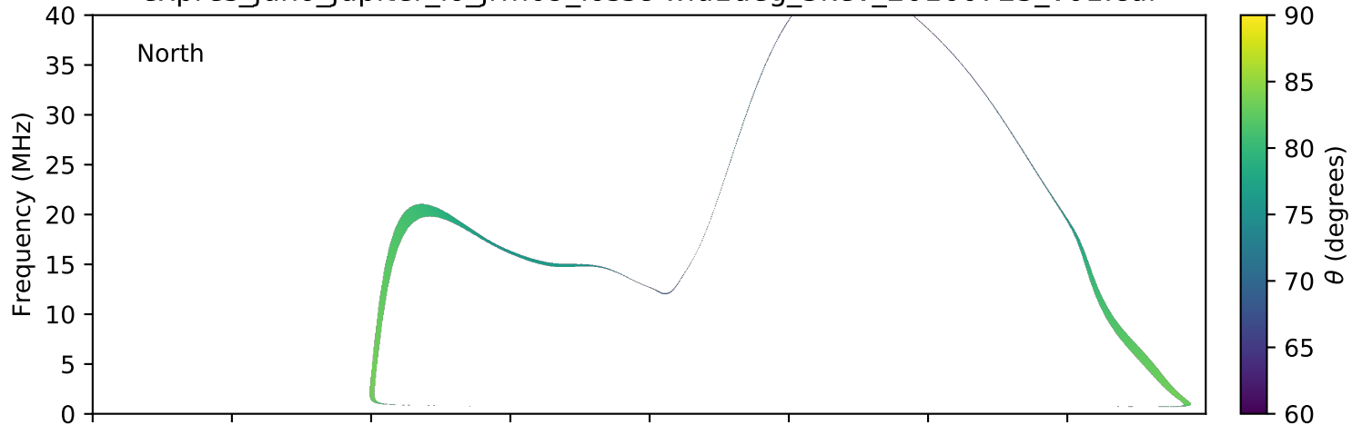
expres_juno_jupiter_io_jrm09_lossc-wid1deg_3kev_20160723_v01.cdf
