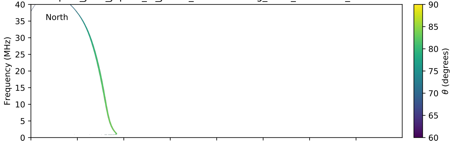
expres_juno_jupiter_io_jrm09_lossc-wid1deg_3kev_20160722_v01.cdf
